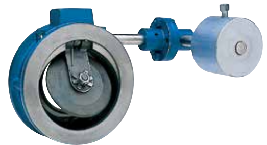
counterweight
